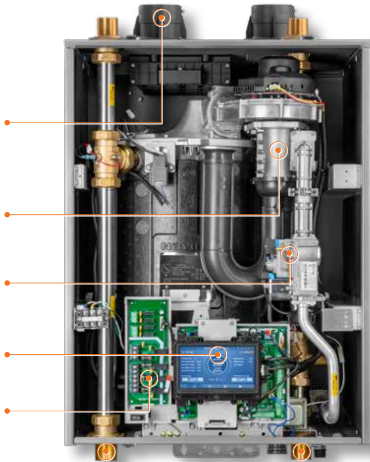
Top and bottom piping
